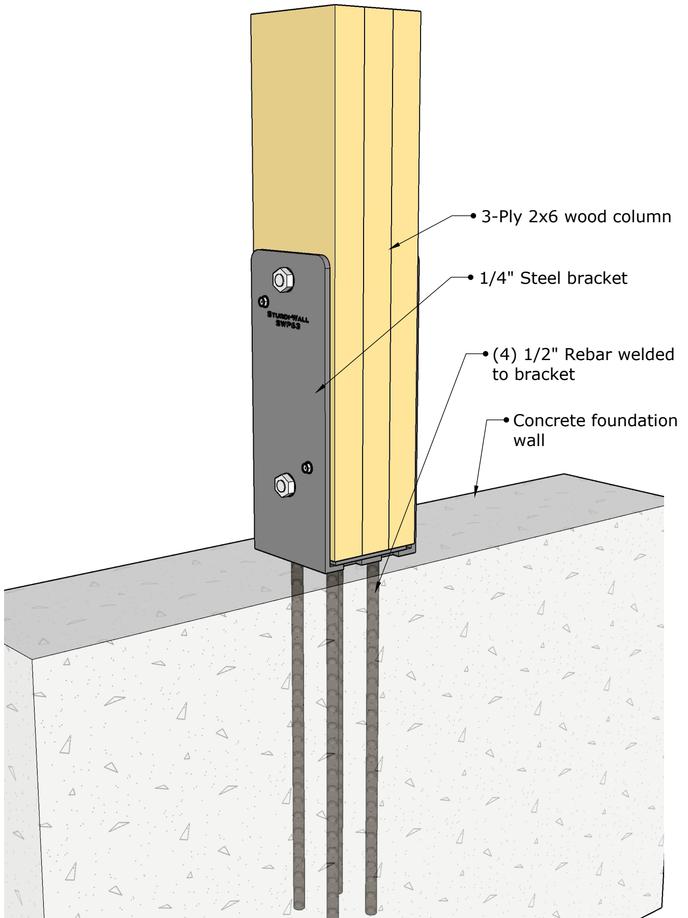
STURDI-WALL PLUS BRACKET SWP63
