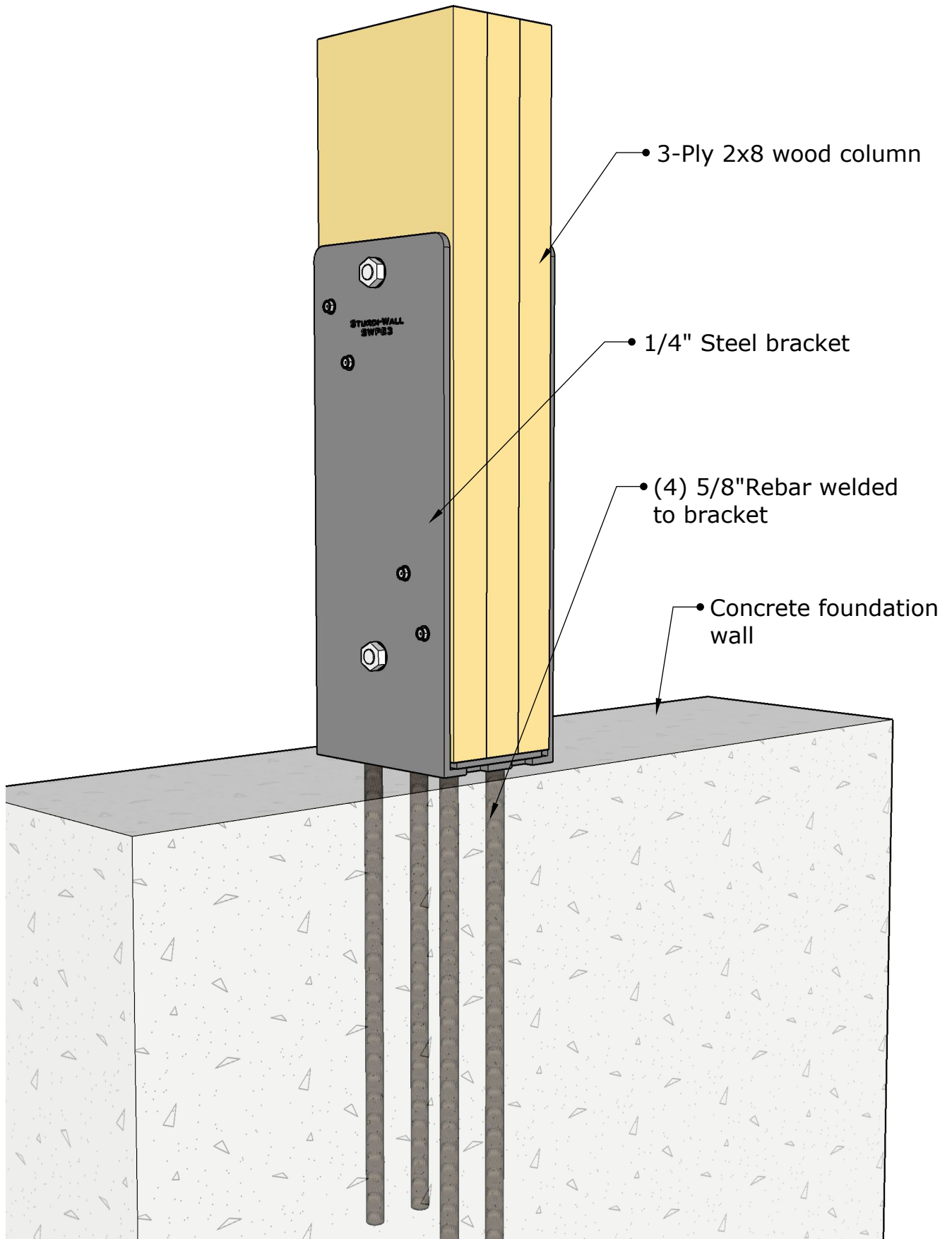
STURDI-WALL PLUS BRACKET SWP83
