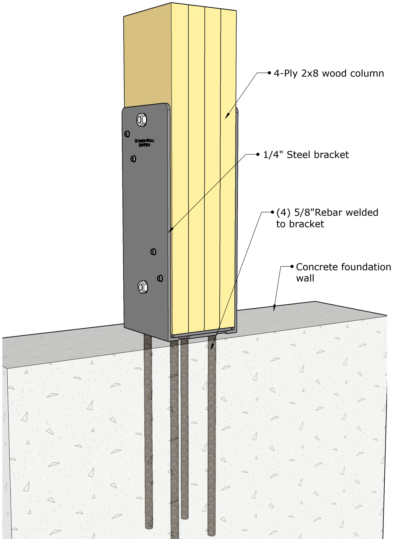
STURDI-WALL PLUS BRACKET SWP84
