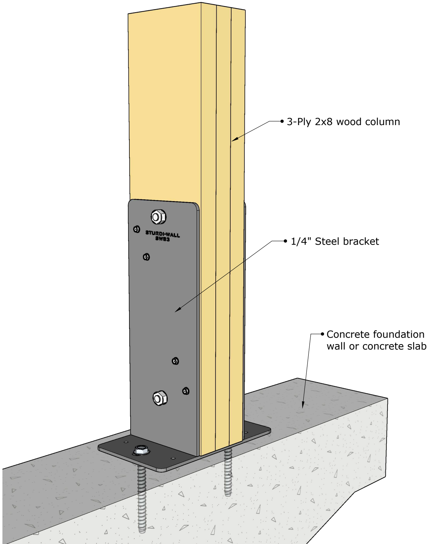
STURDI-WALL BRACKET SW83
